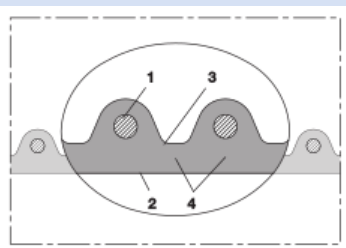
Antistatic food hose and pharmaceutical hose, super-heavy, stainless steel (INOX)
