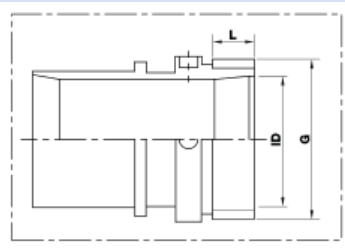
Threaded adapter
