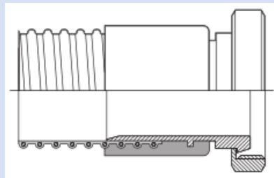
air tube support based on DIN 2826/11851
