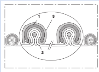
Exhaust gas hose, vibration resistant, outer protection profile
