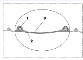
TPE hose, light (up to +150°C)
